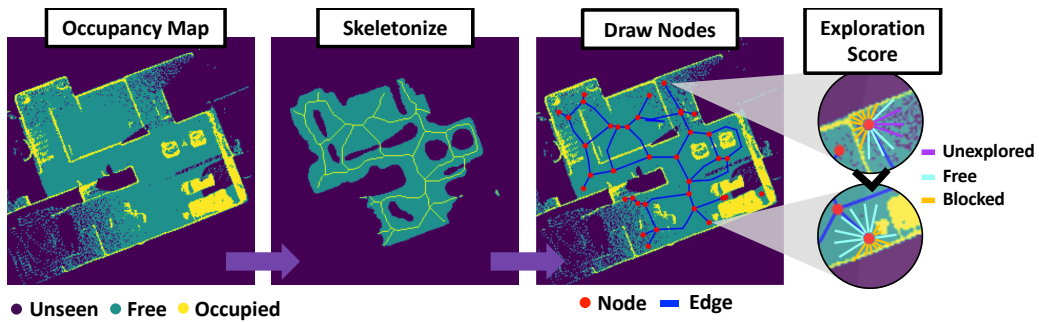
Figure 13. Overview of the graph generation. We take the free area of the occupancy map and skeletonized the image. Then, we draw a graph on the skeleton. Each node has an exploration score, which is calculated based on the number of unseen pixels in the neighborhood.
