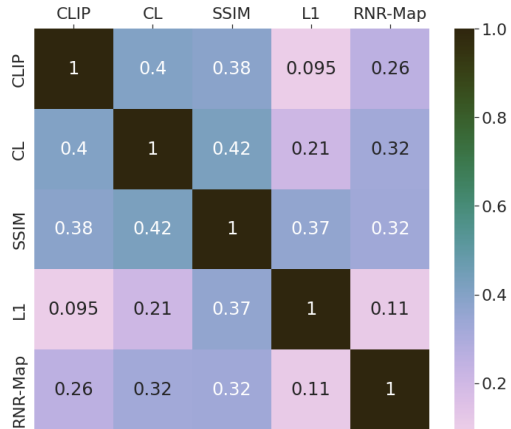
Figure 10. Correlation matrix of the similarity metrics and the probability value from RNR-Map.
