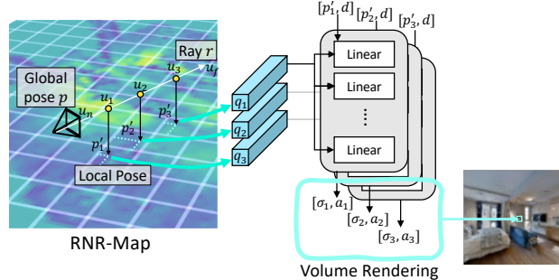
Figure 6. Illustration of decoding process.
